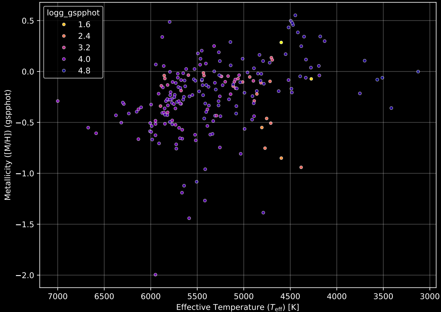
APOGEE DR17 Field: [059-48-O] Stellar Population Parameters (n= 217)
