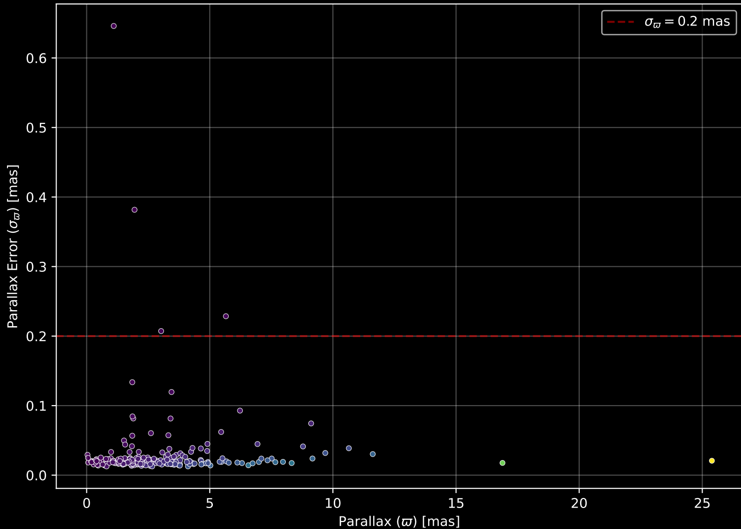
APOGEE DR17 Field: [059-48-O] Parallax Quality (n= 217)
