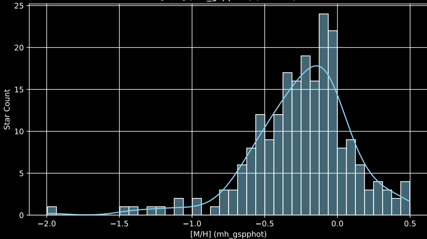
APOGEE DR17 Field: [059-48-O [M/H] (mh_gspphot) (n= 216)
