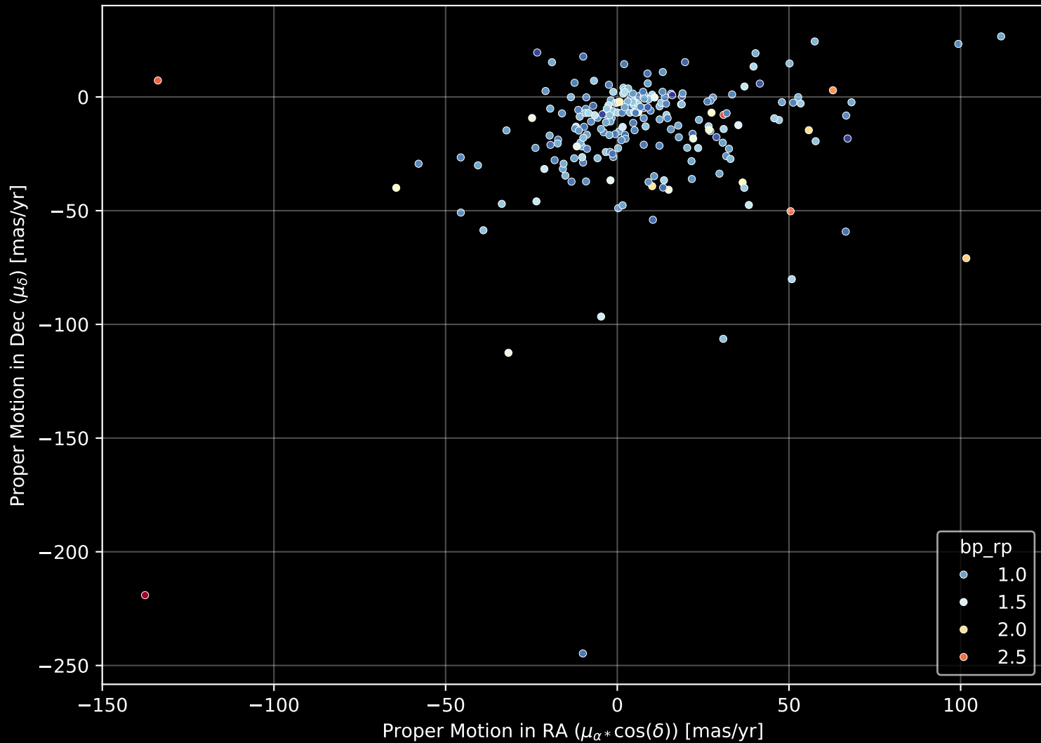
APOGEE DR17 Field: [059-48-O] Proper Motion Diagram (n= 217)
