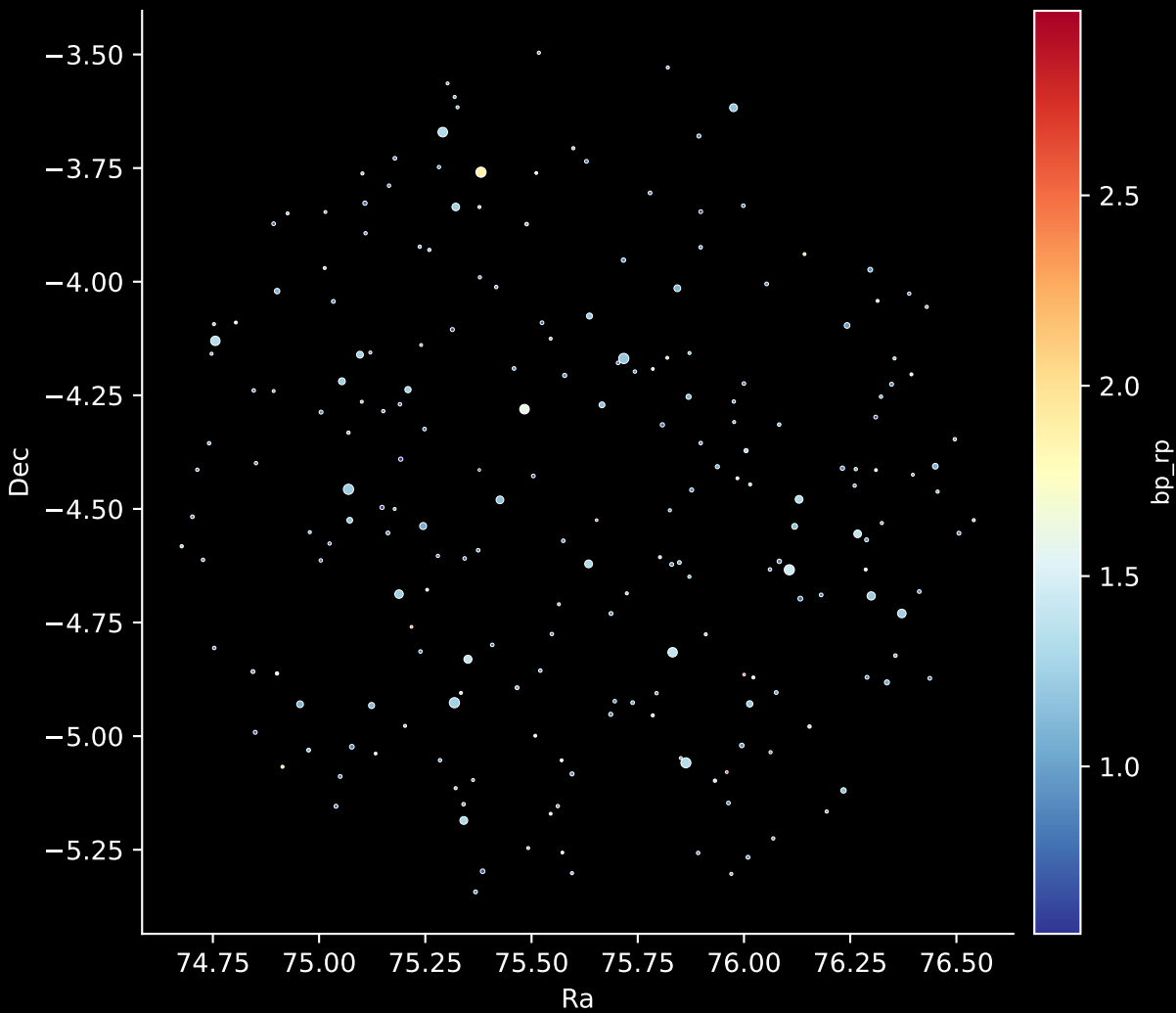
APOGEE DR17 Field: [059-48-O] Stars: 217
