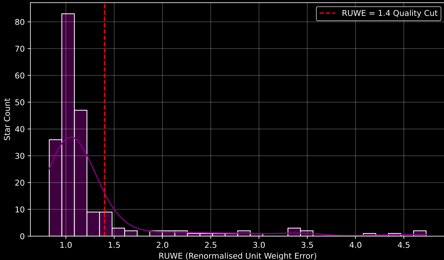
GAPOGEE DR17 Field [059-48-O] RUWE Distribution (n= 211)
