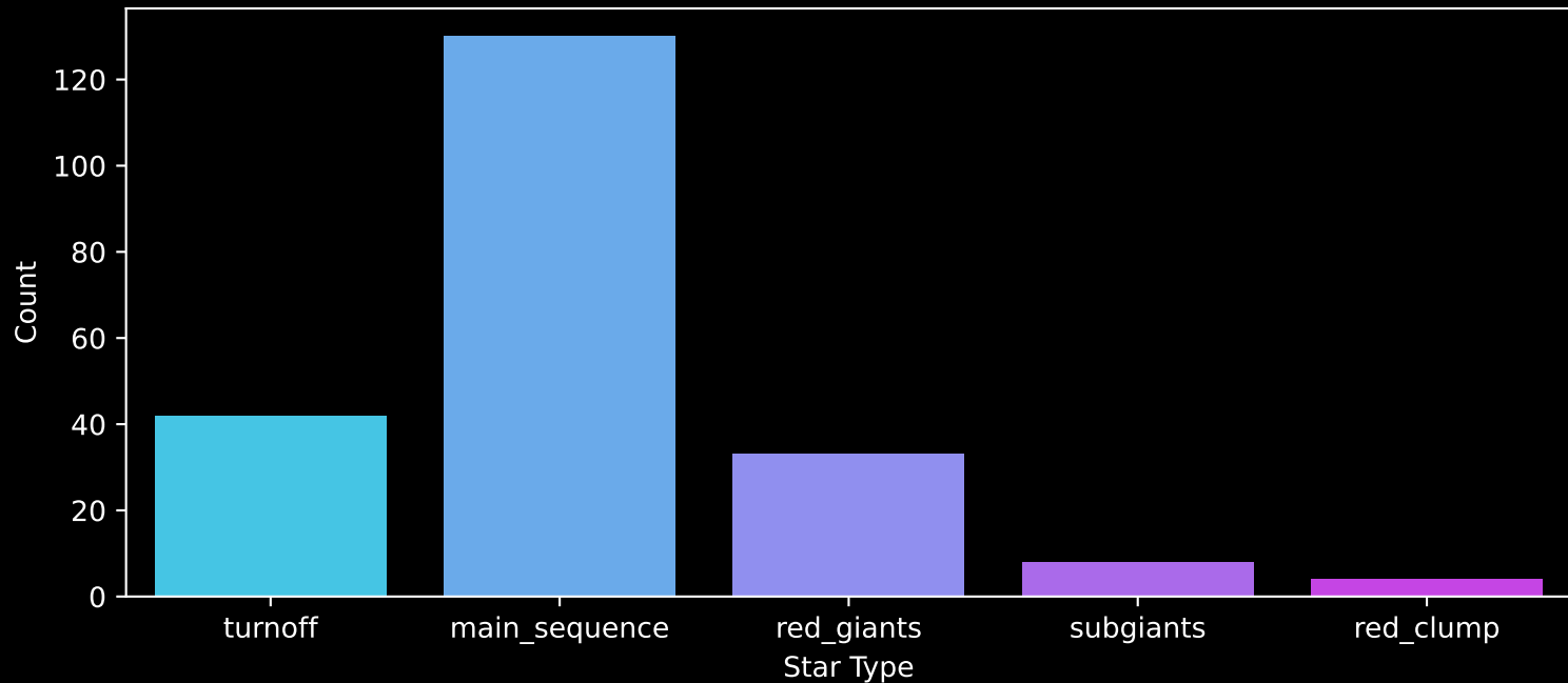
APOGEE DR17 Field: [059-48-O] Count plot of Star Type
